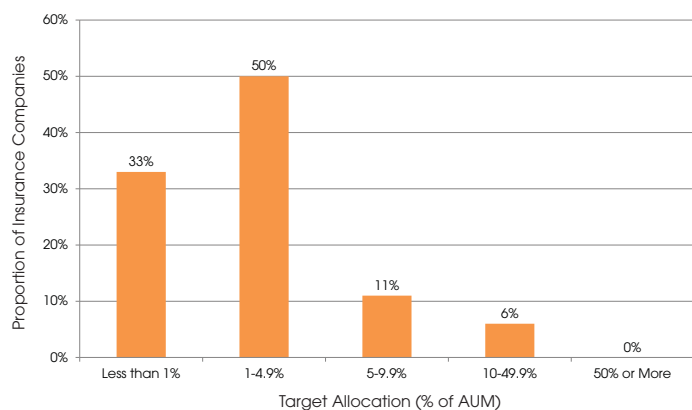
Fig. 3: Breakdown of Insurance Companies Investing in Infrastructure by Target Allocation (As a % of Total Assets)
